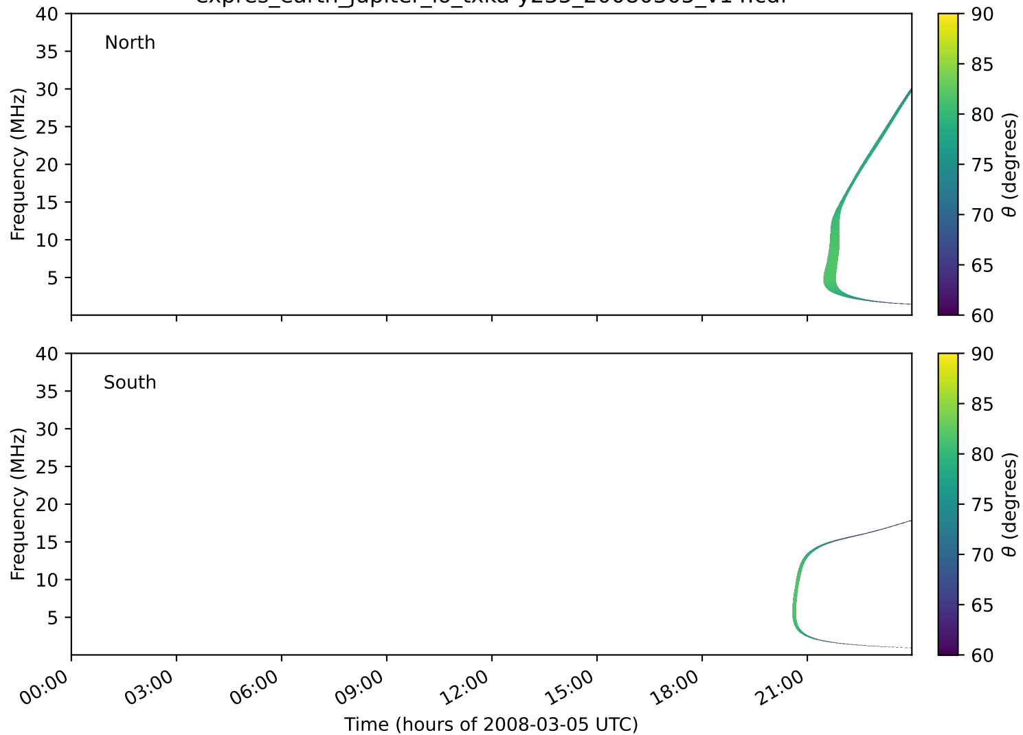
expres_earth_jupiter_io_txka-y235_20080305_v14.cdf
