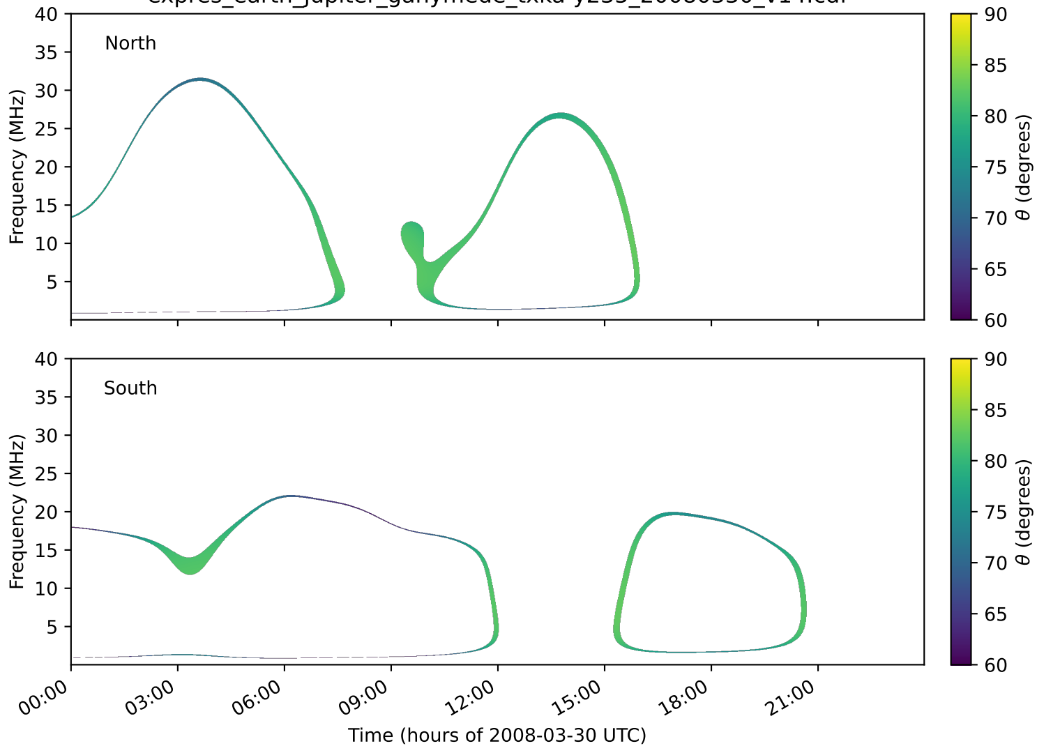
expres_earth_jupiter_ganymede_txka-y235_20080330_v14.cdf
