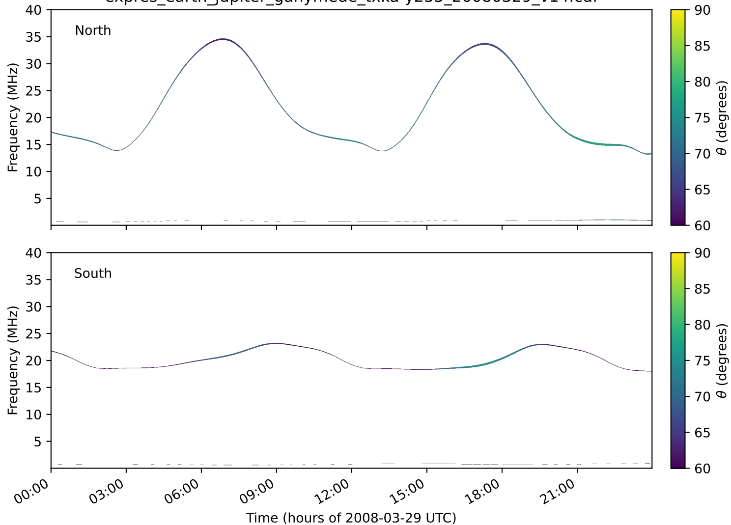
expres_earth_jupiter_ganymede_txka-y235_20080329_v14.cdf
