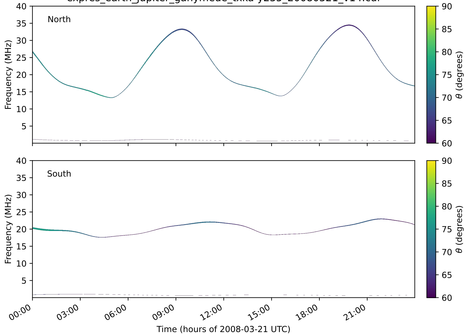
expres_earth_jupiter_ganymede_txka-y235_20080321_v14.cdf
