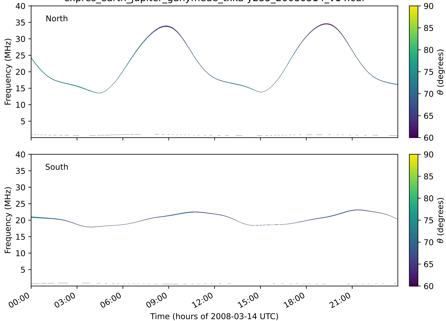
expres_earth_jupiter_ganymede_txka-y235_20080314_v14.cdf
