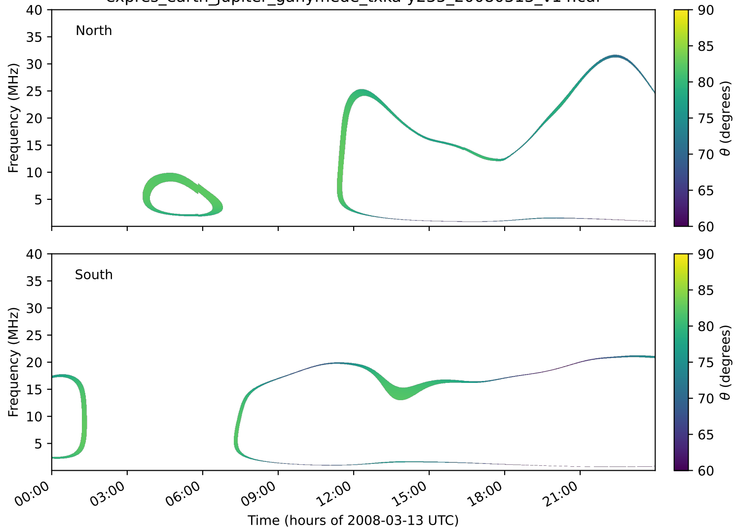
expres_earth_jupiter_ganymede_txka-y235_20080313_v14.cdf
