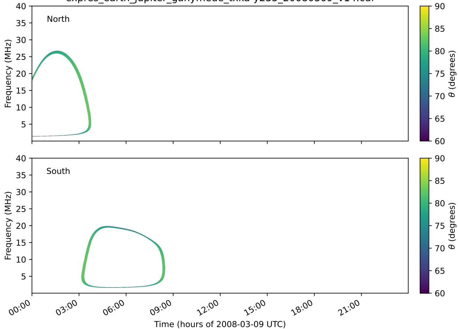
expres_earth_jupiter_ganymede_txka-y235_20080309_v14.cdf
