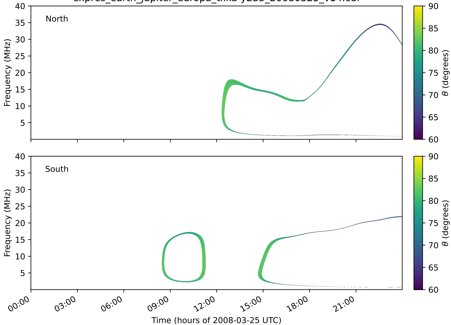
expres_earth_jupiter_europa_txka-y235_20080325_v14.cdf
