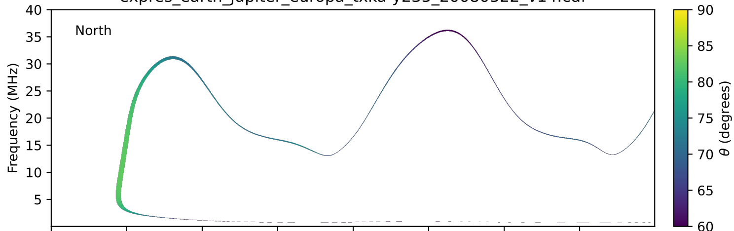
expres_earth_jupiter_europa_txka-y235_20080322_v14.cdf
