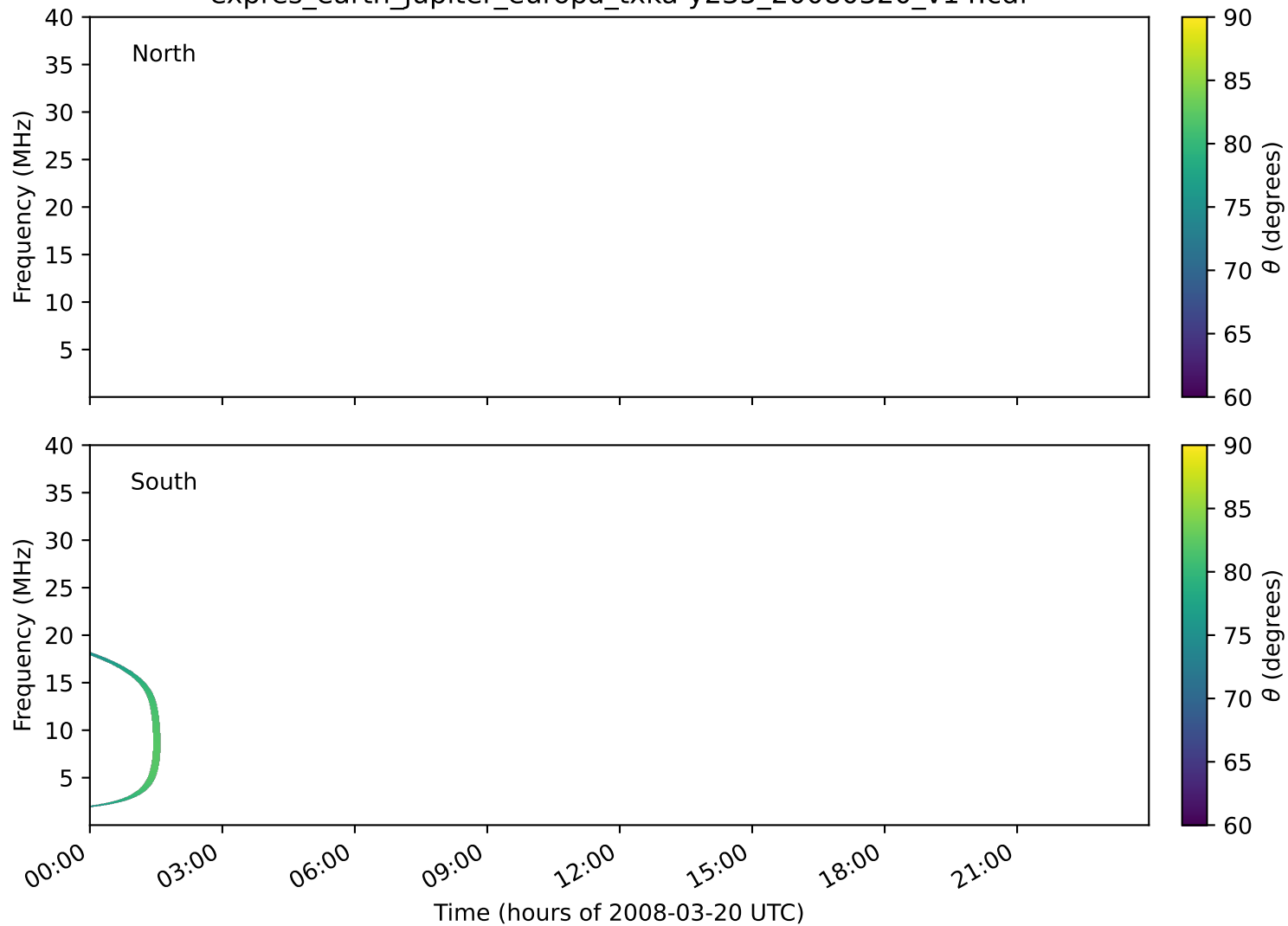
expres_earth_jupiter_europa_txka-y235_20080320_v14.cdf
