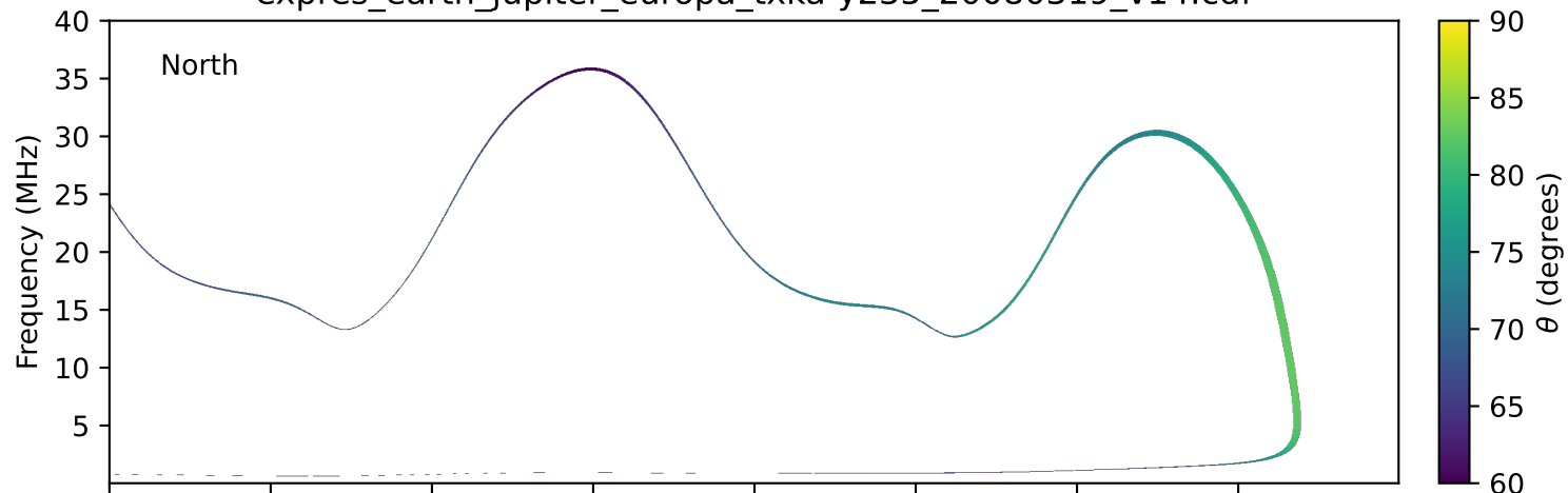
expres_earth_jupiter_europa_txka-y235_20080319_v14.cdf
