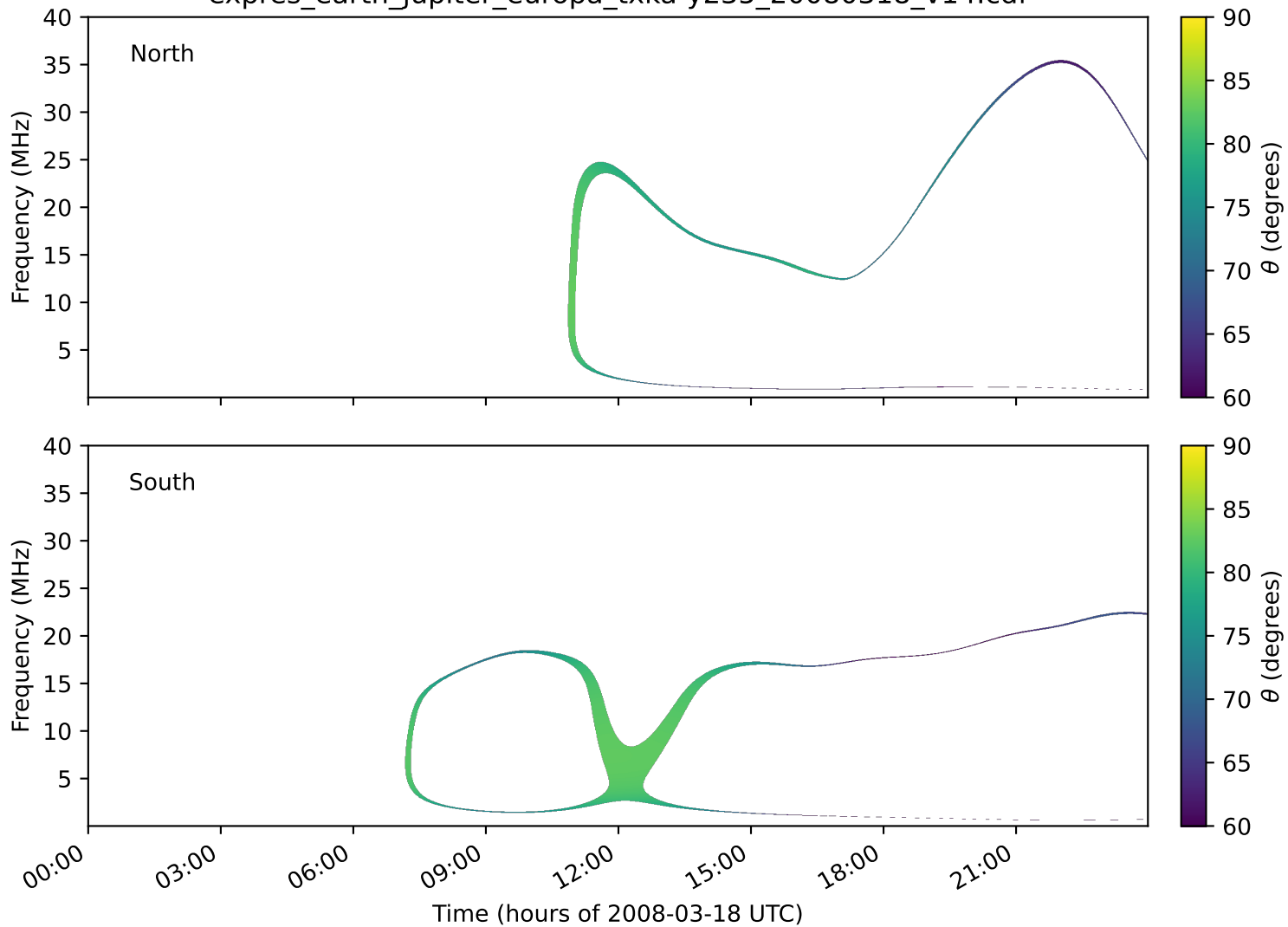
expres_earth_jupiter_europa_txka-y235_20080318_v14.cdf
