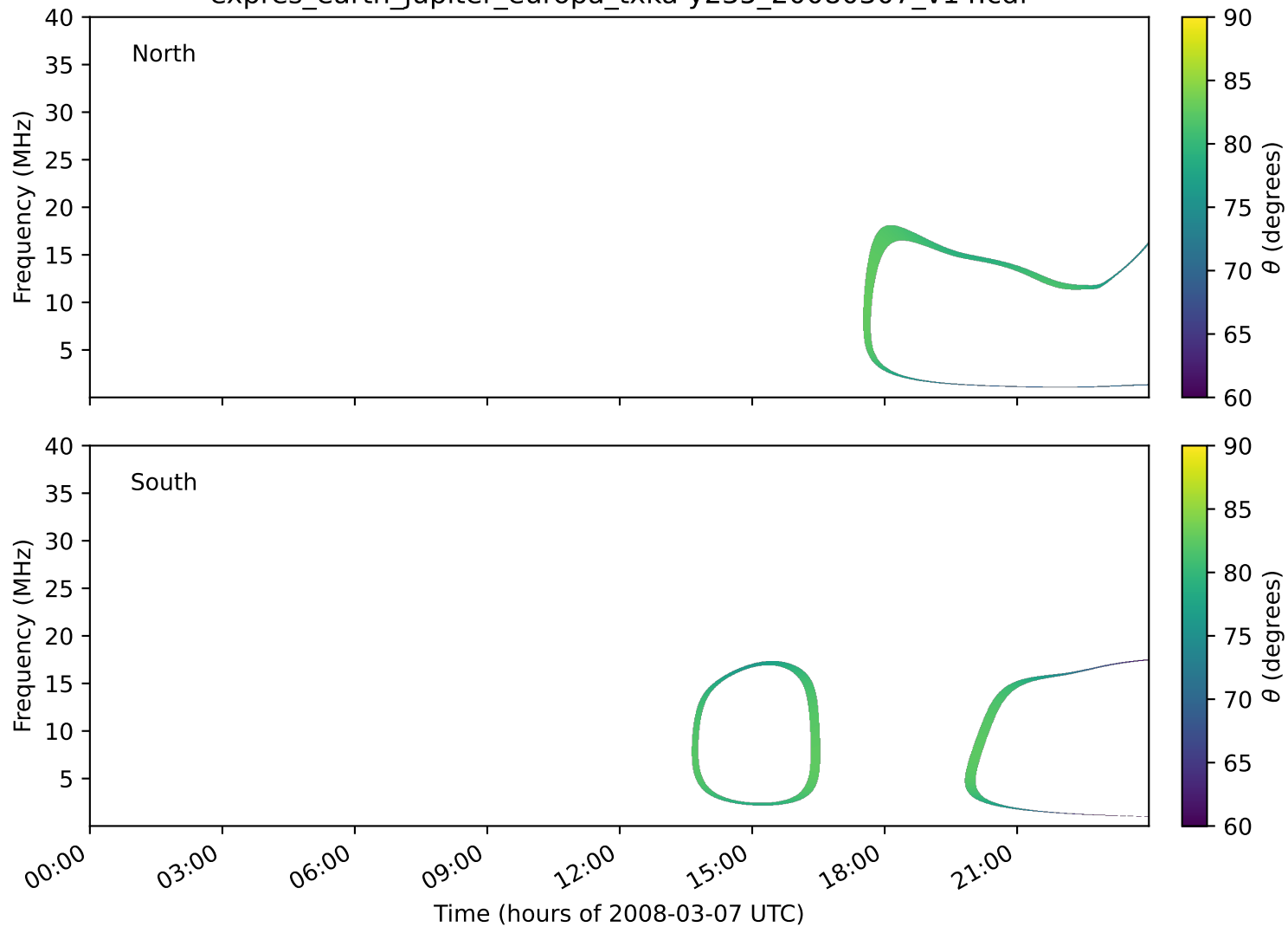
expres_earth_jupiter_europa_txka-y235_20080307_v14.cdf
