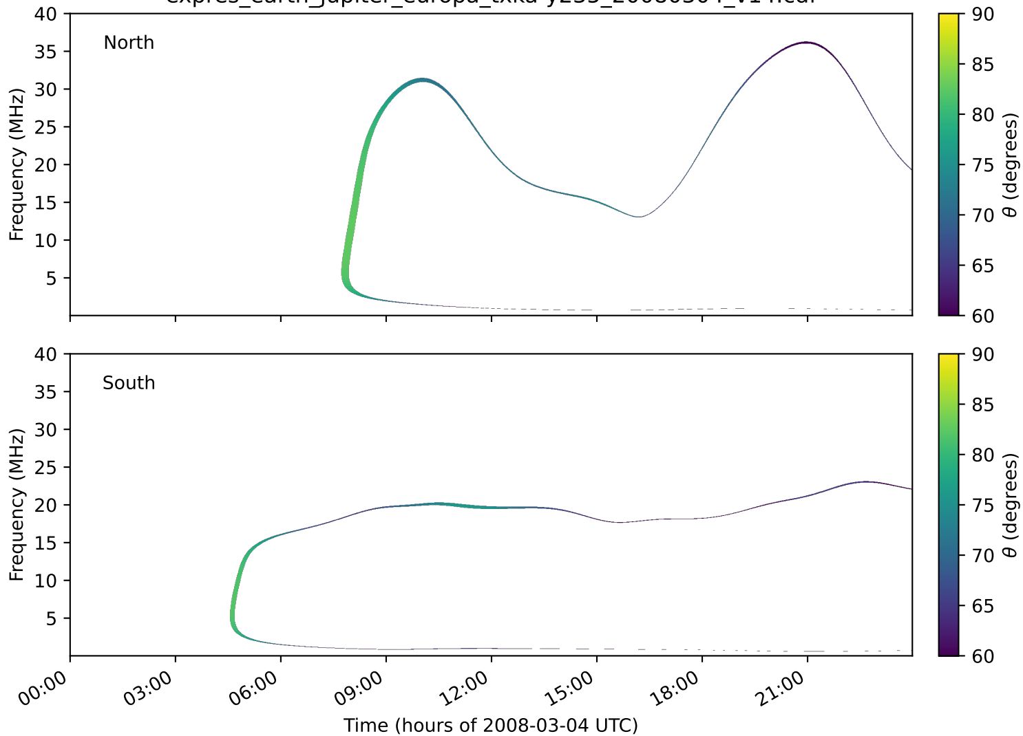
expres_earth_jupiter_europa_txka-y235_20080304_v14.cdf
