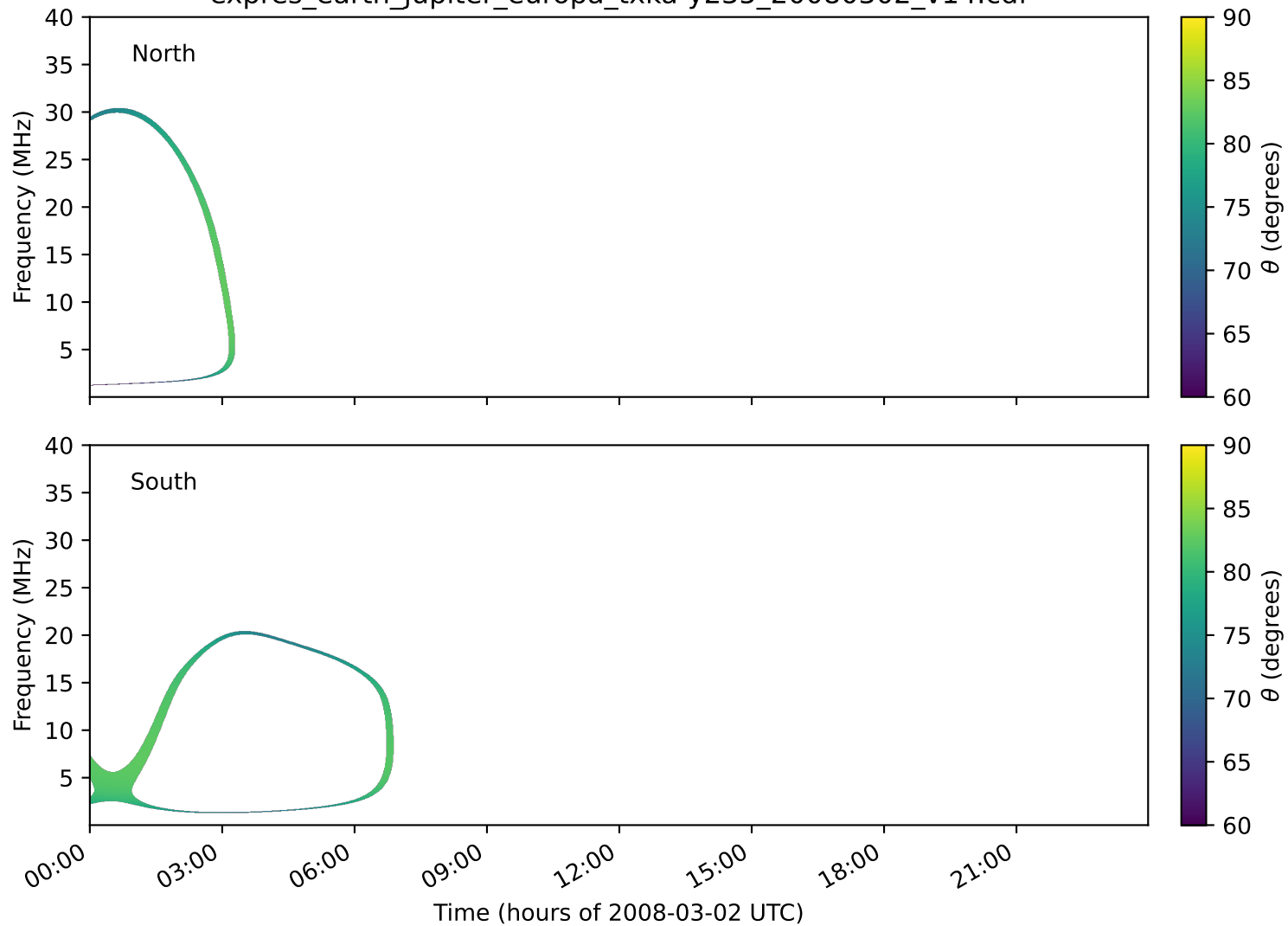
expres_earth_jupiter_europa_txka-y235_20080302_v14.cdf
