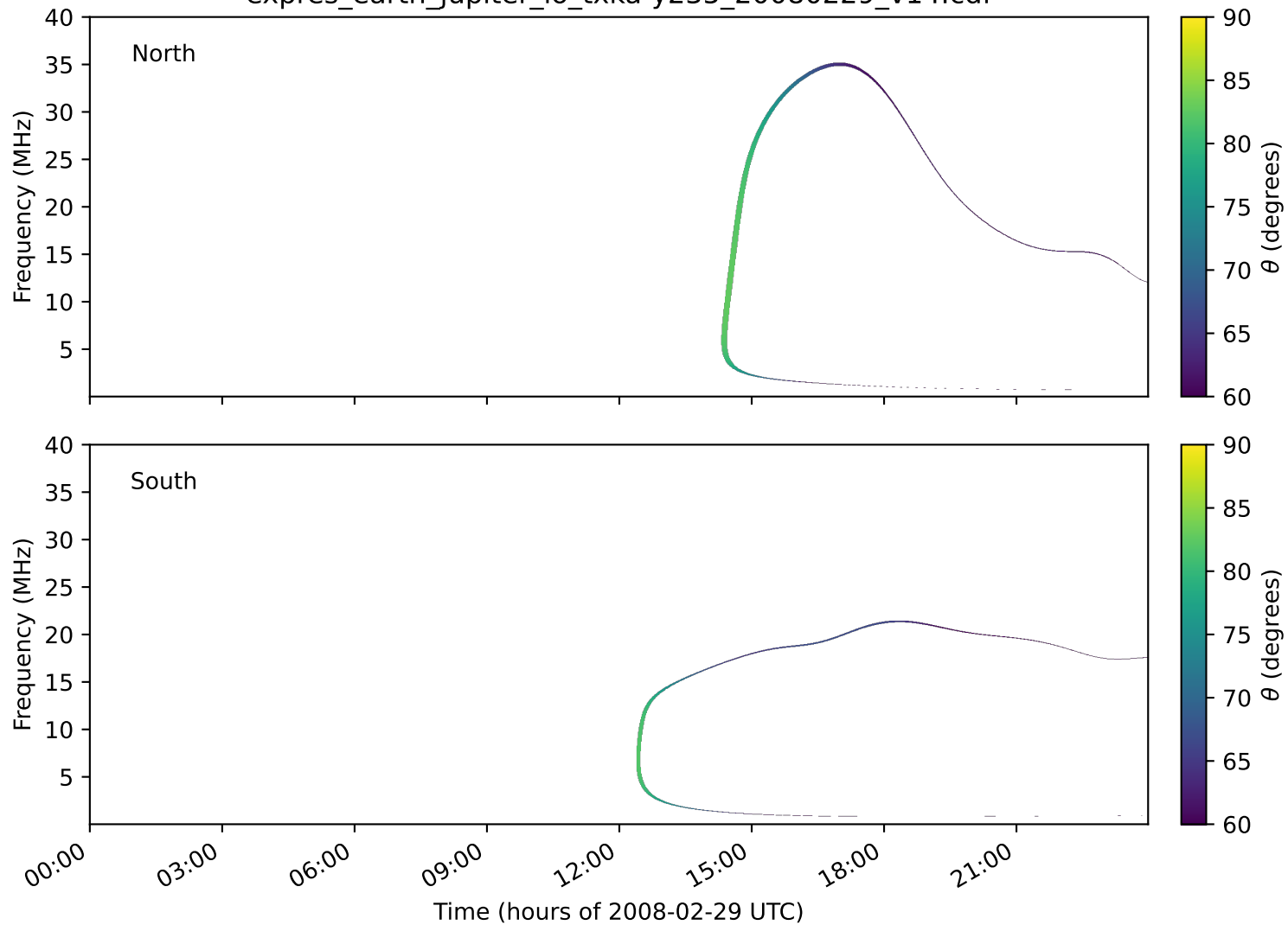
expres_earth_jupiter_io_txka-y235_20080229_v14.cdf
