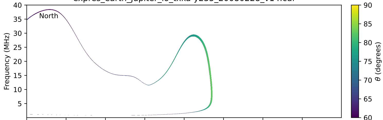
expres_earth_jupiter_io_txka-y235_20080228_v14.cdf
