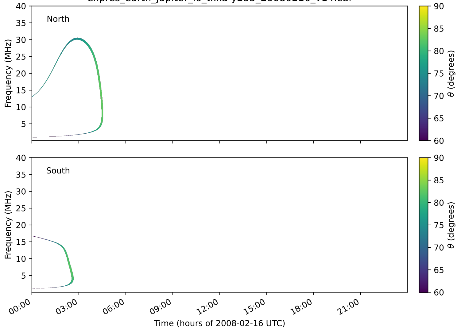
expres_earth_jupiter_io_txka-y235_20080216_v14.cdf
