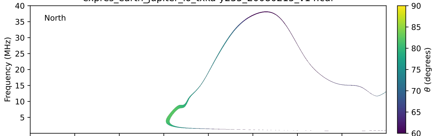
expres_earth_jupiter_io_txka-y235_20080215_v14.cdf
