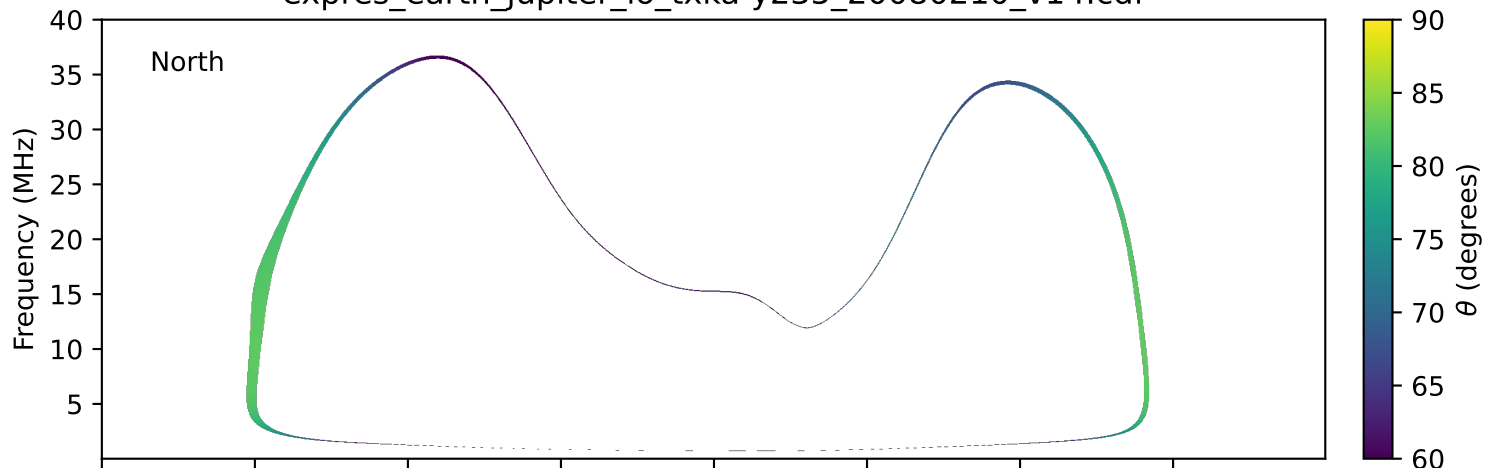
expres_earth_jupiter_io_txka-y235_20080210_v14.cdf
