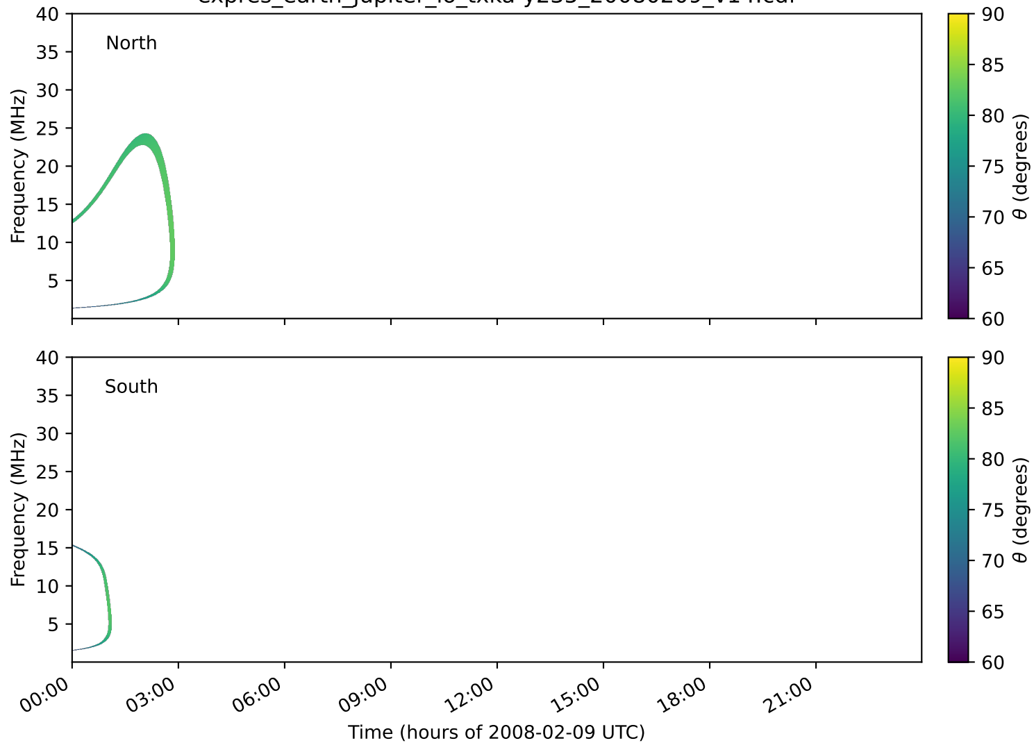
expres_earth_jupiter_io_txka-y235_20080209_v14.cdf
