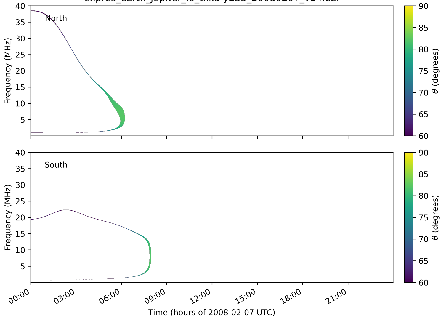
expres_earth_jupiter_io_txka-y235_20080207_v14.cdf
