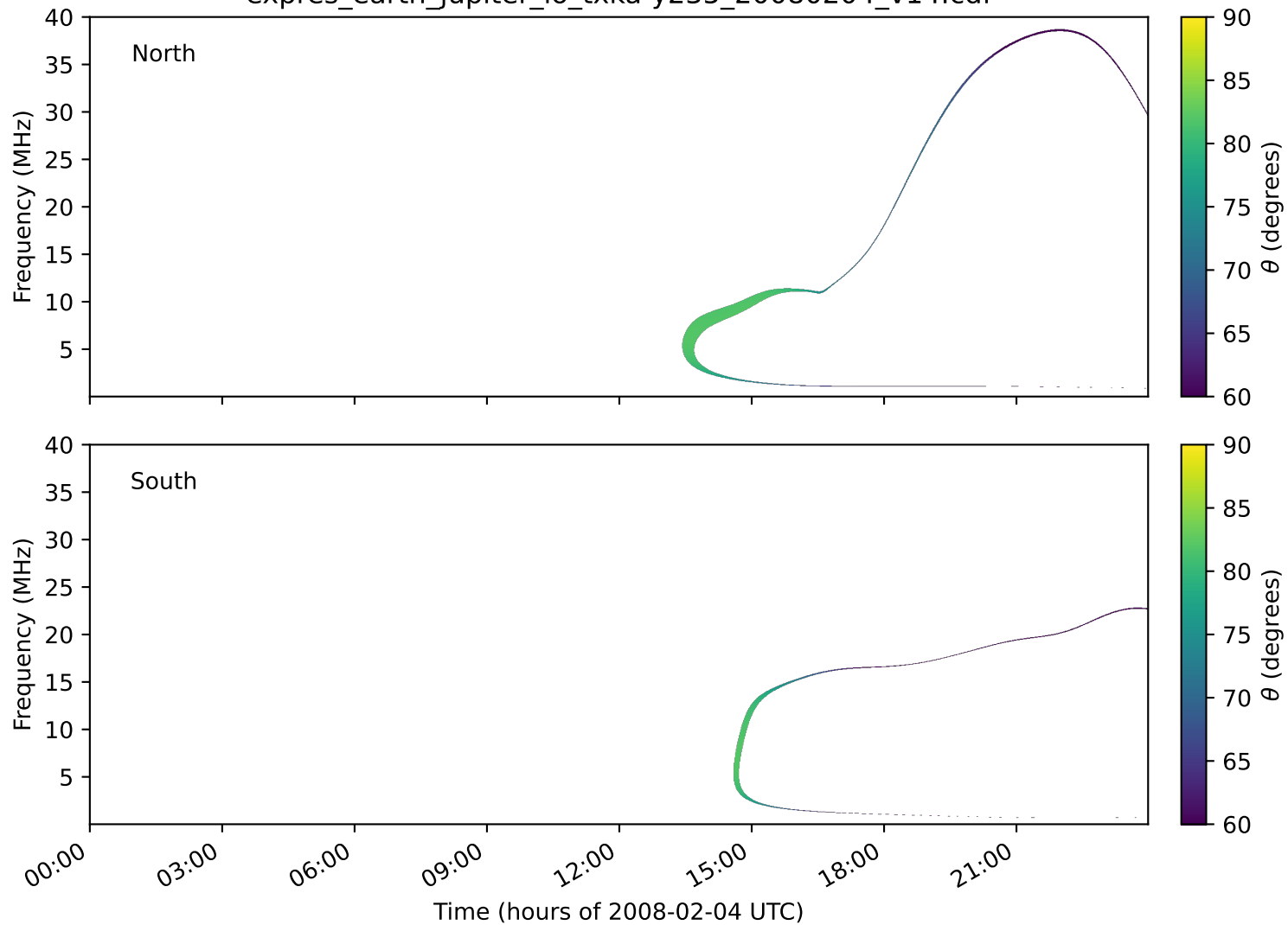
expres_earth_jupiter_io_txka-y235_20080204_v14.cdf
