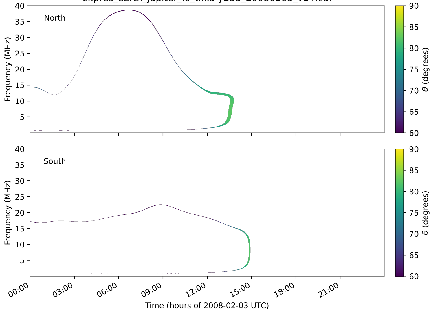
expres_earth_jupiter_io_txka-y235_20080203_v14.cdf
