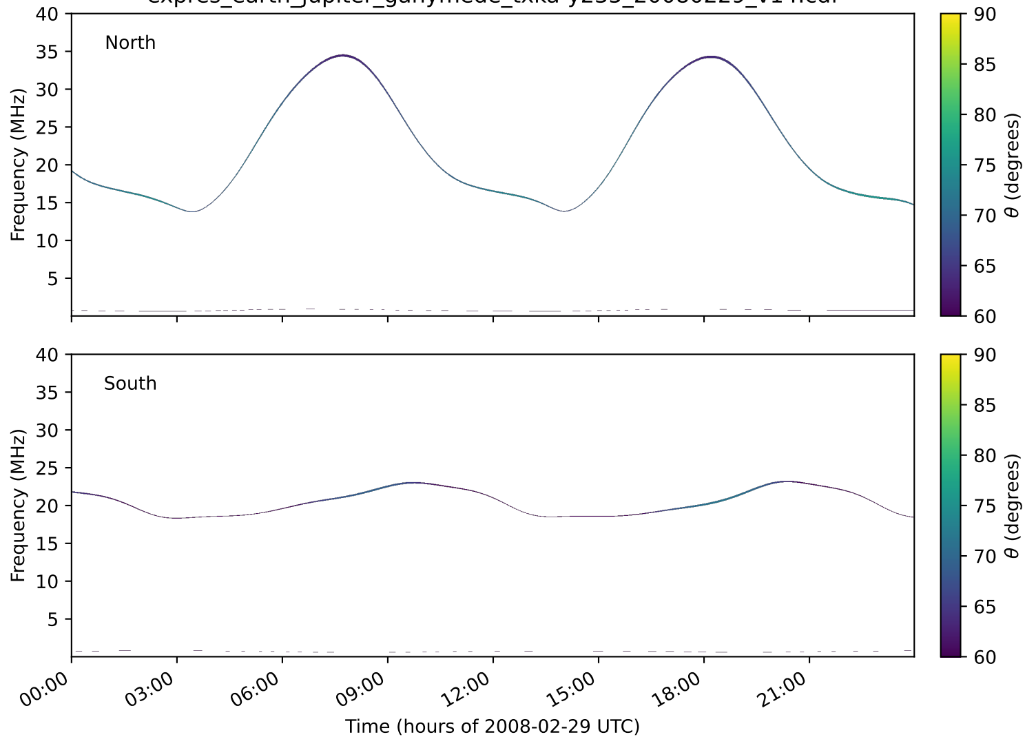
expres_earth_jupiter_ganymede_txka-y235_20080229_v14.cdf
