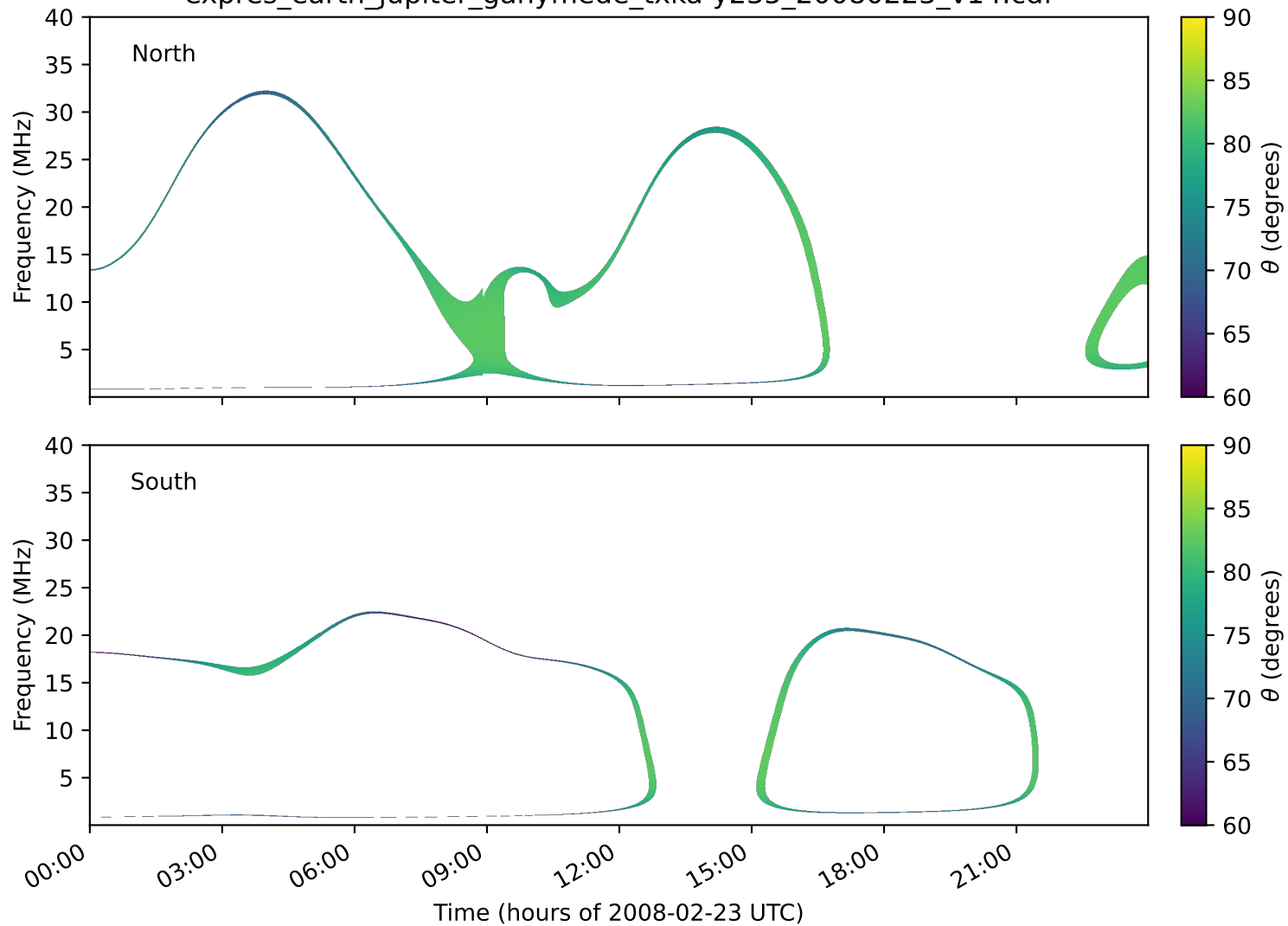
expres_earth_jupiter_ganymede_txka-y235_20080223_v14.cdf
