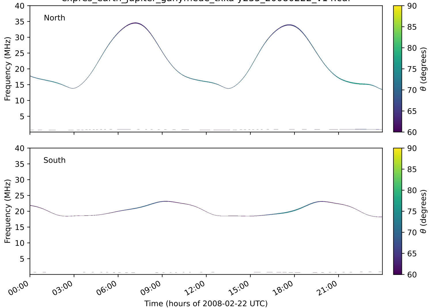
expres_earth_jupiter_ganymede_txka-y235_20080222_v14.cdf
