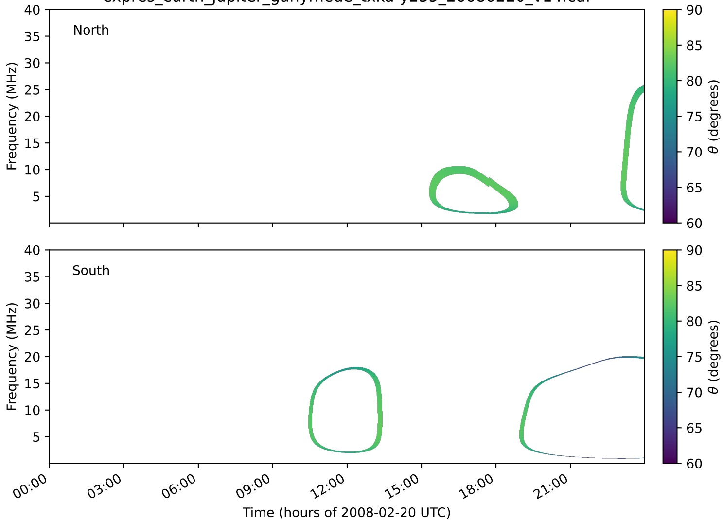
expres_earth_jupiter_ganymede_txka-y235_20080220_v14.cdf
