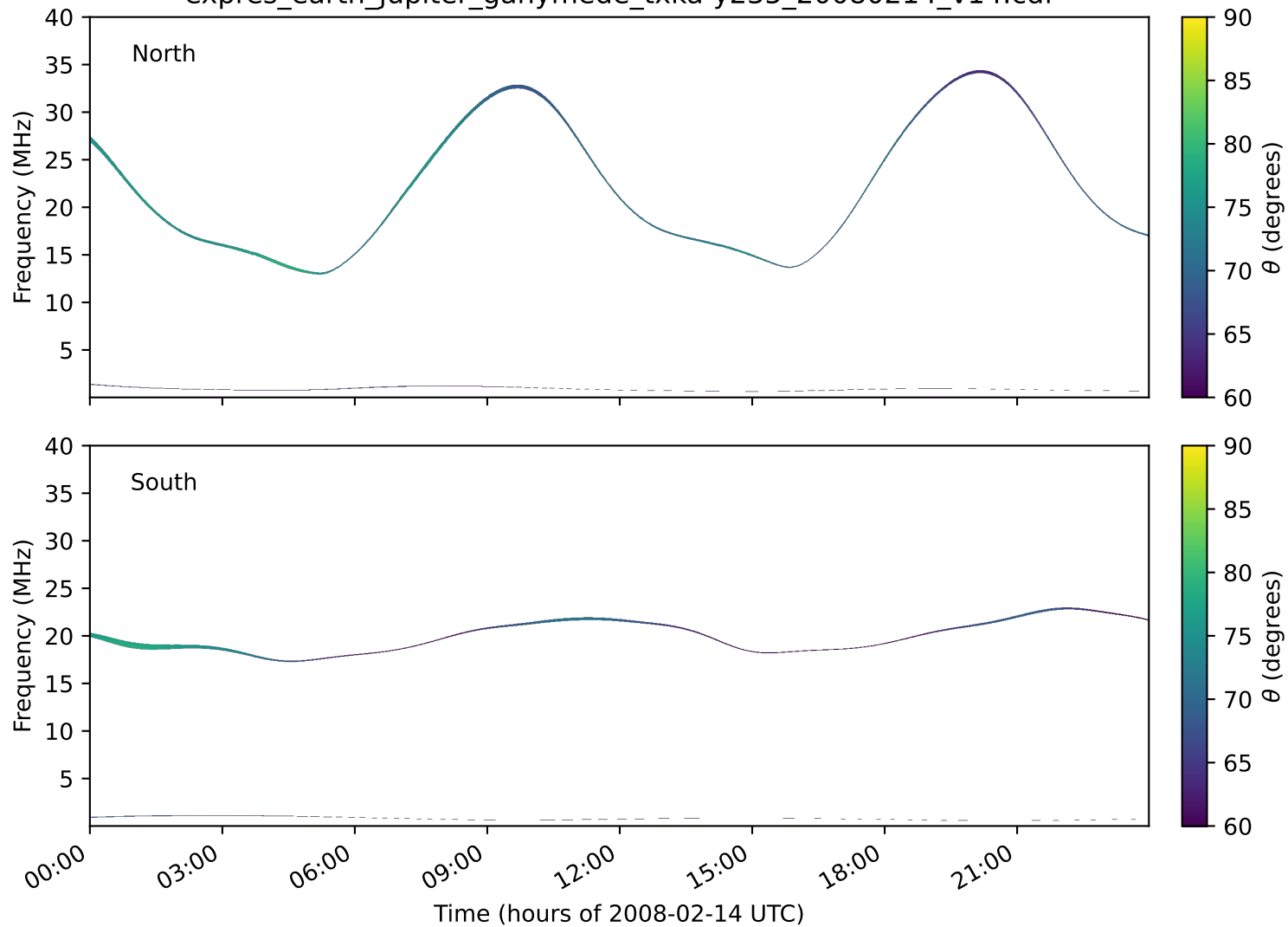
expres_earth_jupiter_ganymede_txka-y235_20080214_v14.cdf
