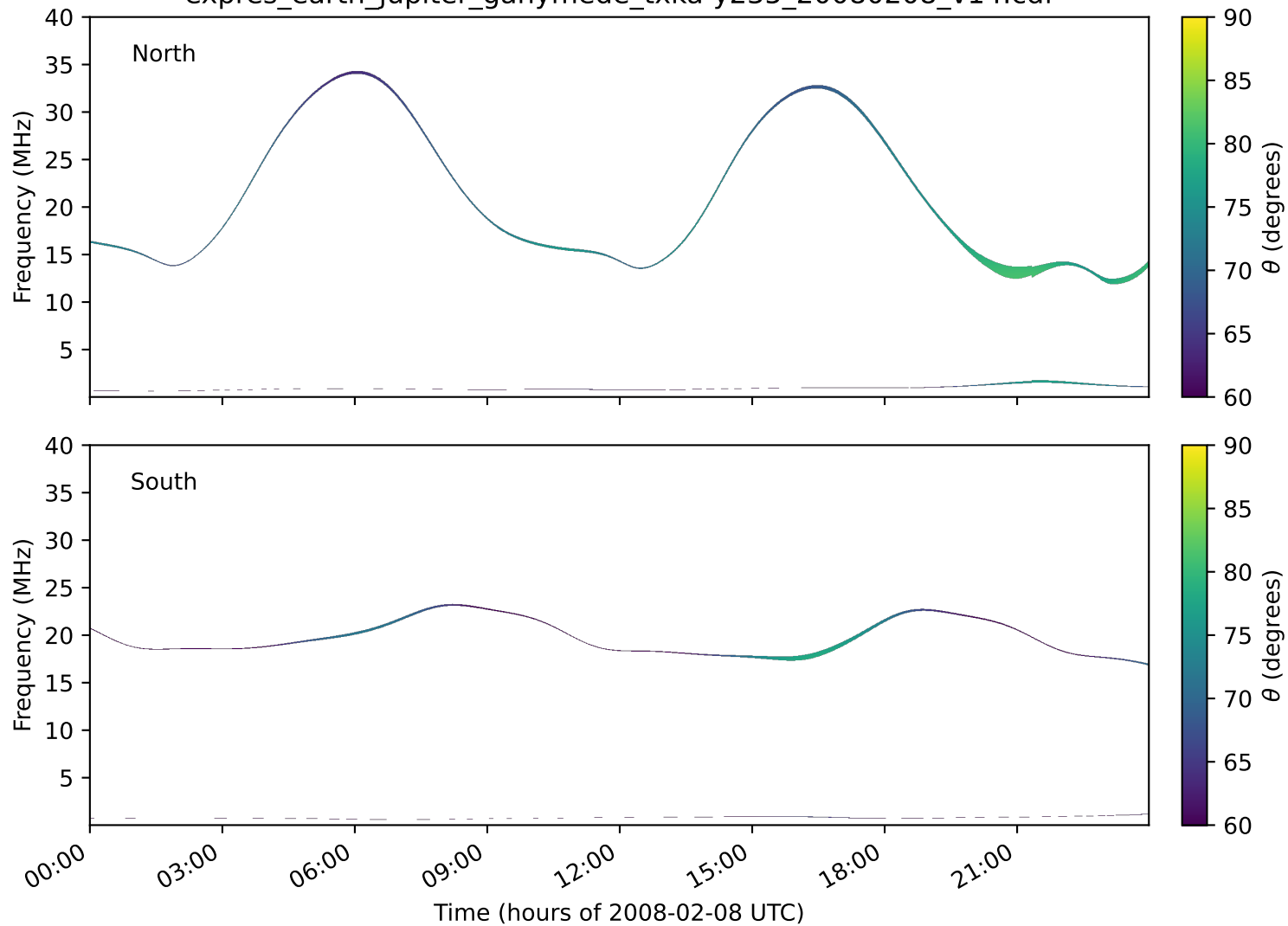
expres_earth_jupiter_ganymede_txka-y235_20080208_v14.cdf
