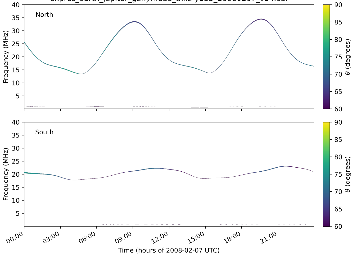
expres_earth_jupiter_ganymede_txka-y235_20080207_v14.cdf
