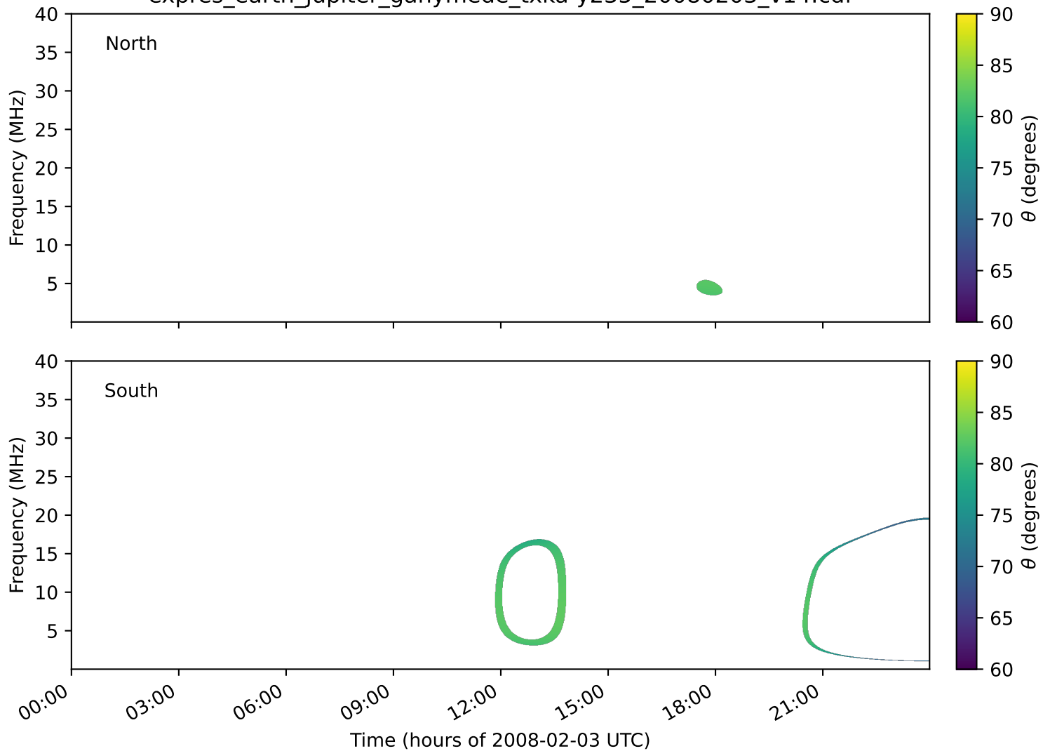
expres_earth_jupiter_ganymede_txka-y235_20080203_v14.cdf
