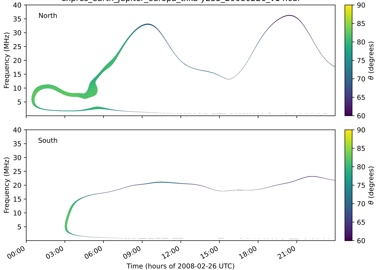
expres_earth_jupiter_europa_txka-y235_20080226_v14.cdf
