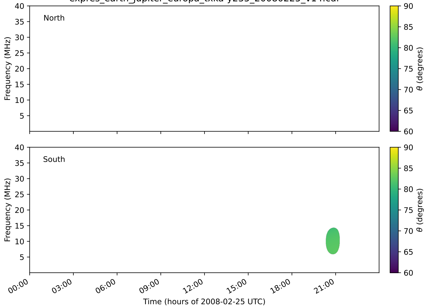
expres_earth_jupiter_europa_txka-y235_20080225_v14.cdf
