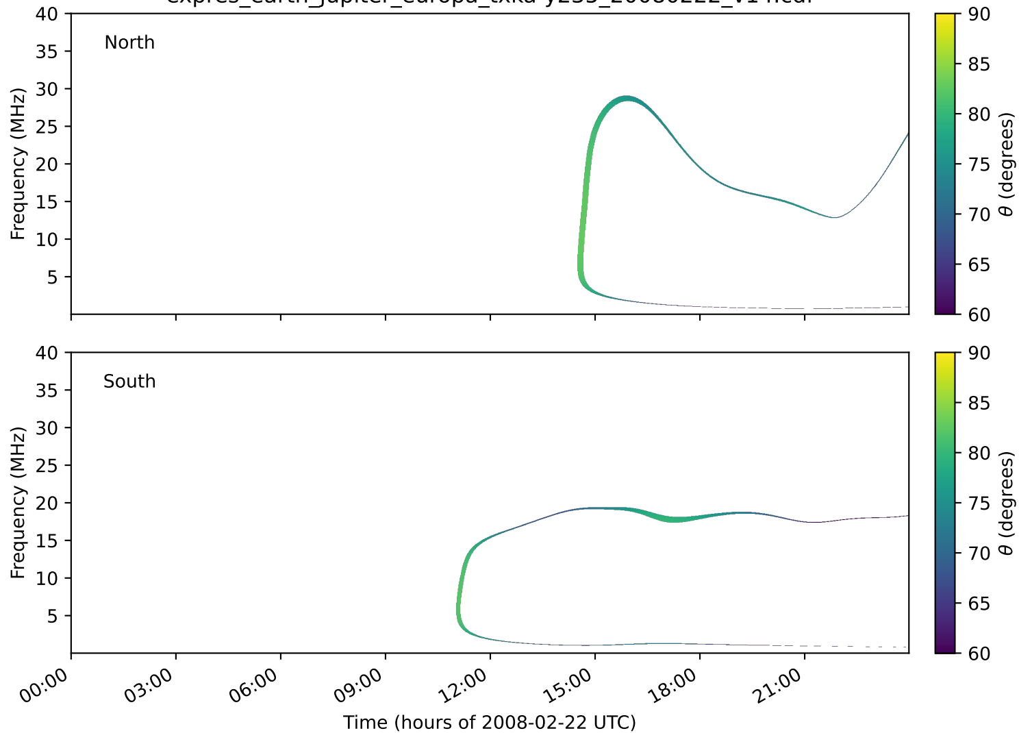
expres_earth_jupiter_europa_txka-y235_20080222_v14.cdf
