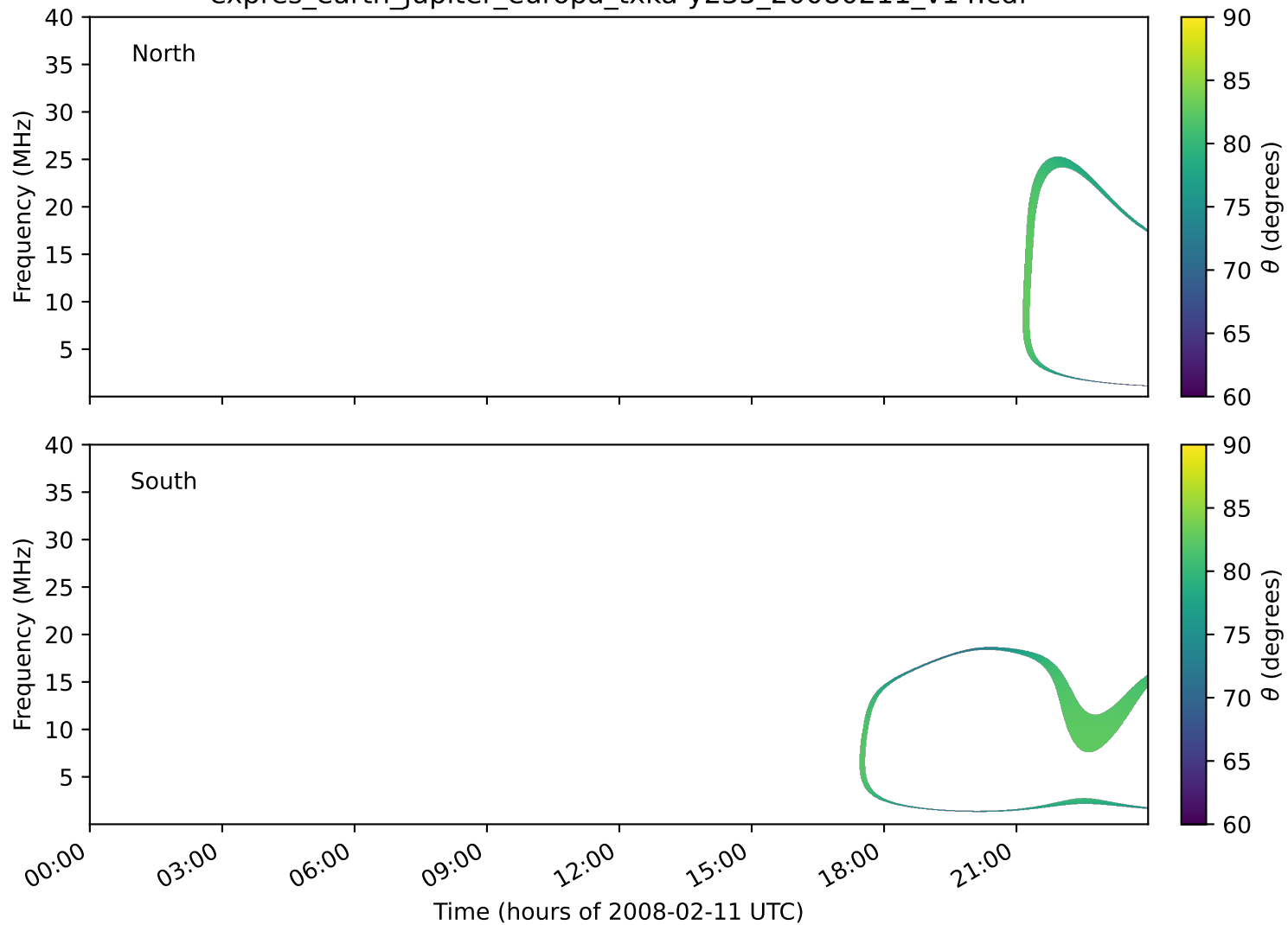
expres_earth_jupiter_europa_txka-y235_20080211_v14.cdf
