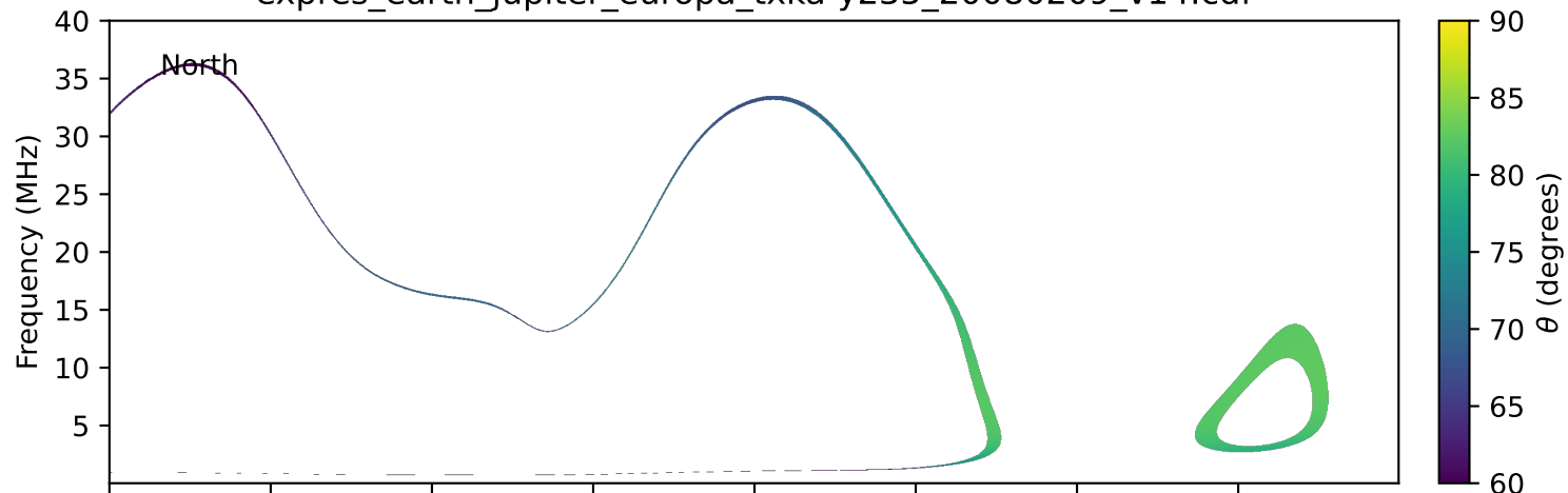
expres_earth_jupiter_europa_txka-y235_20080209_v14.cdf
