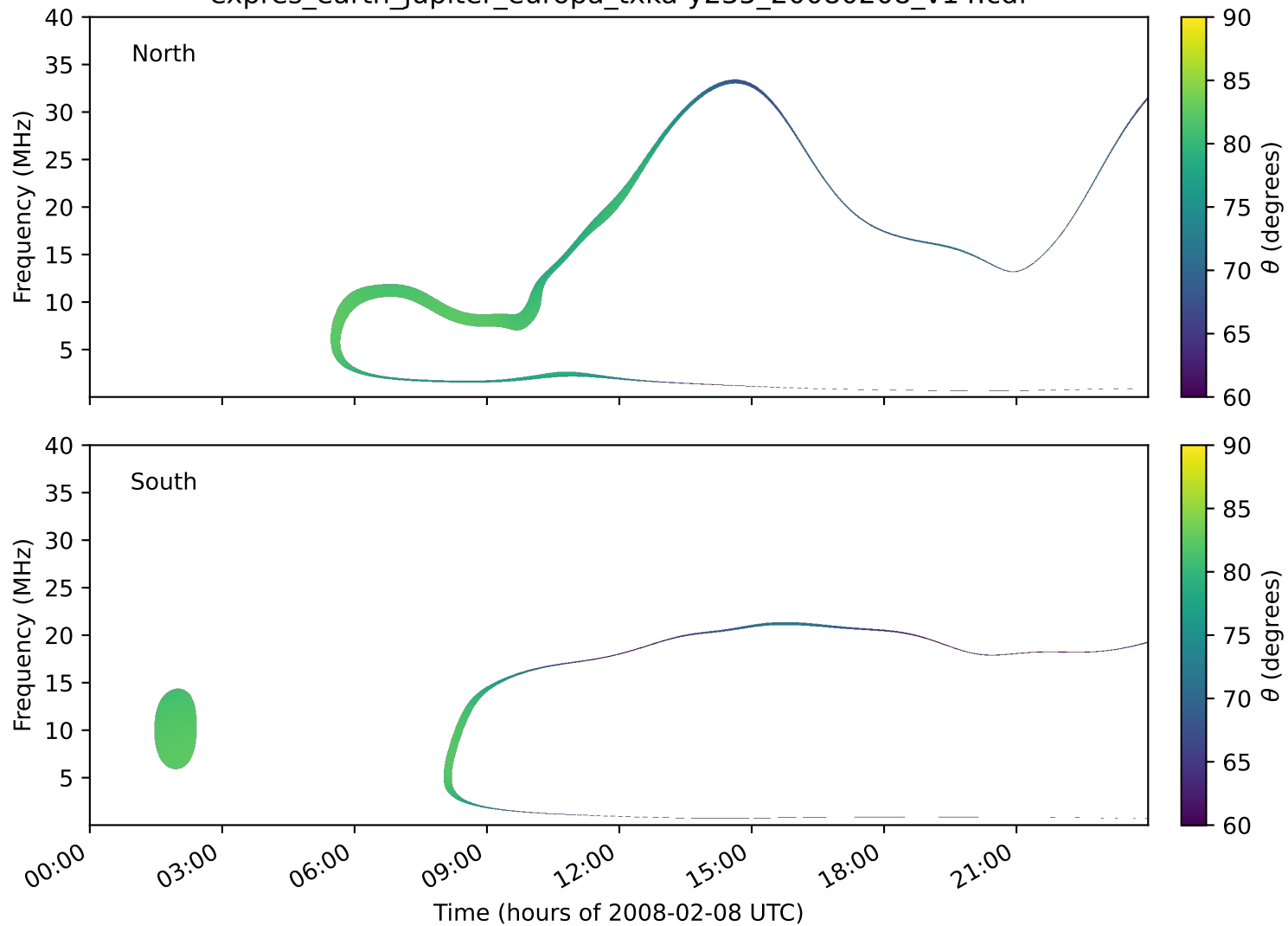
expres_earth_jupiter_europa_txka-y235_20080208_v14.cdf
