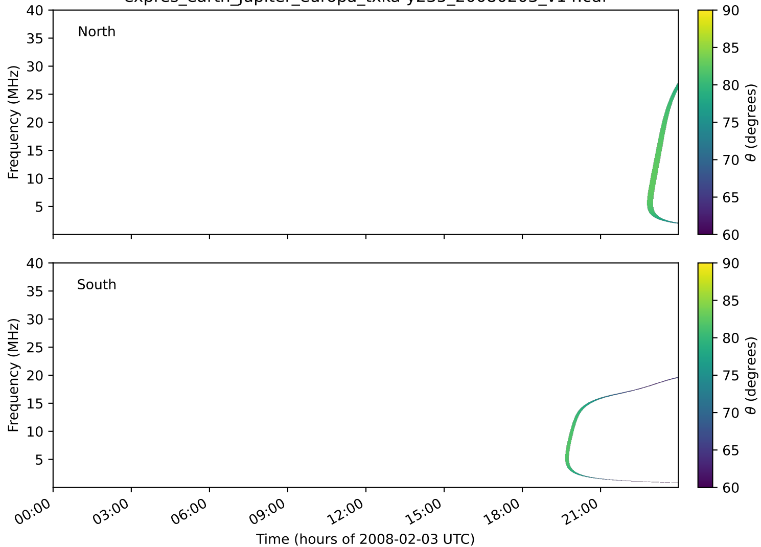
expres_earth_jupiter_europa_txka-y235_20080203_v14.cdf
