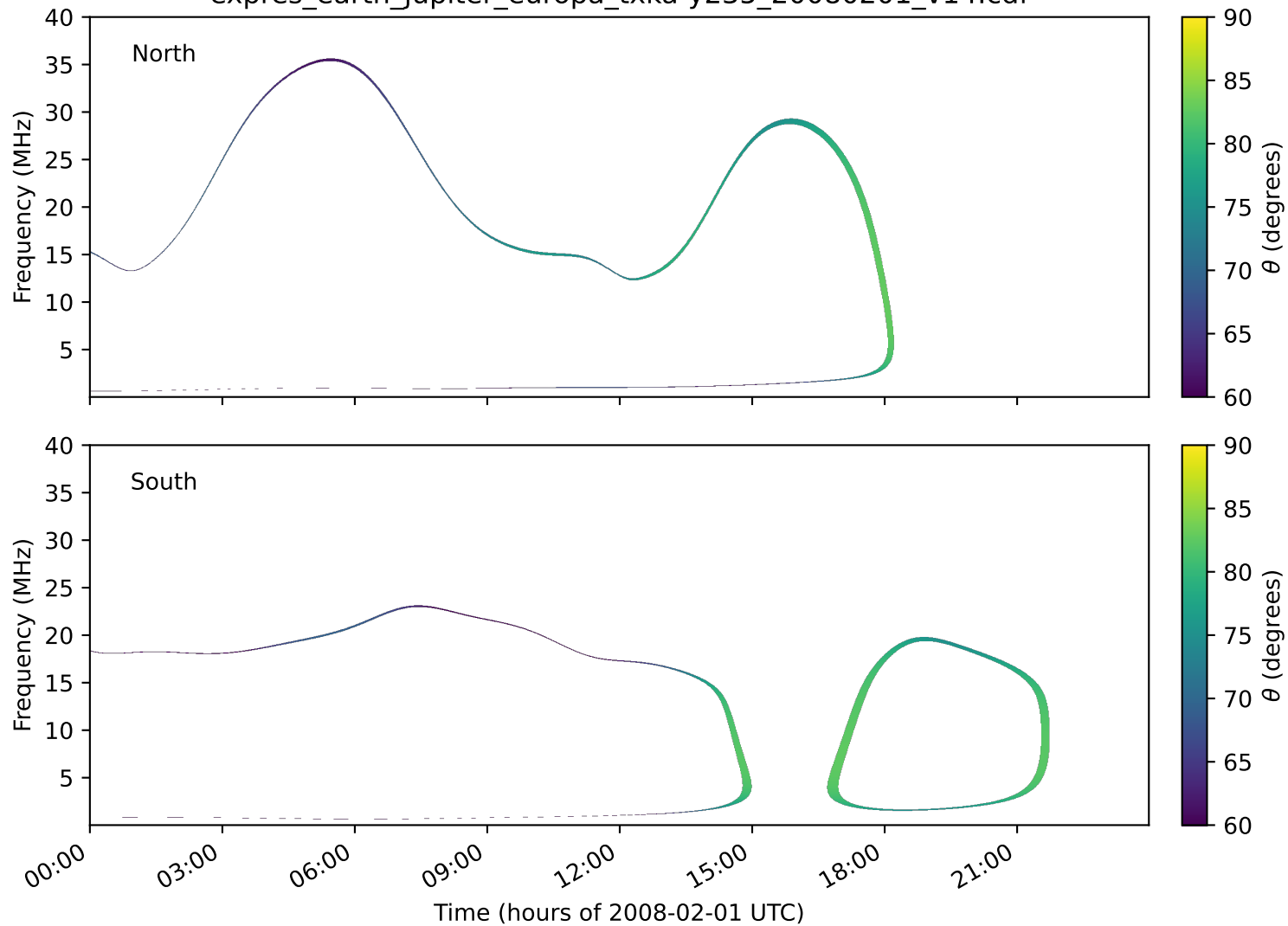
expres_earth_jupiter_europa_txka-y235_20080201_v14.cdf
