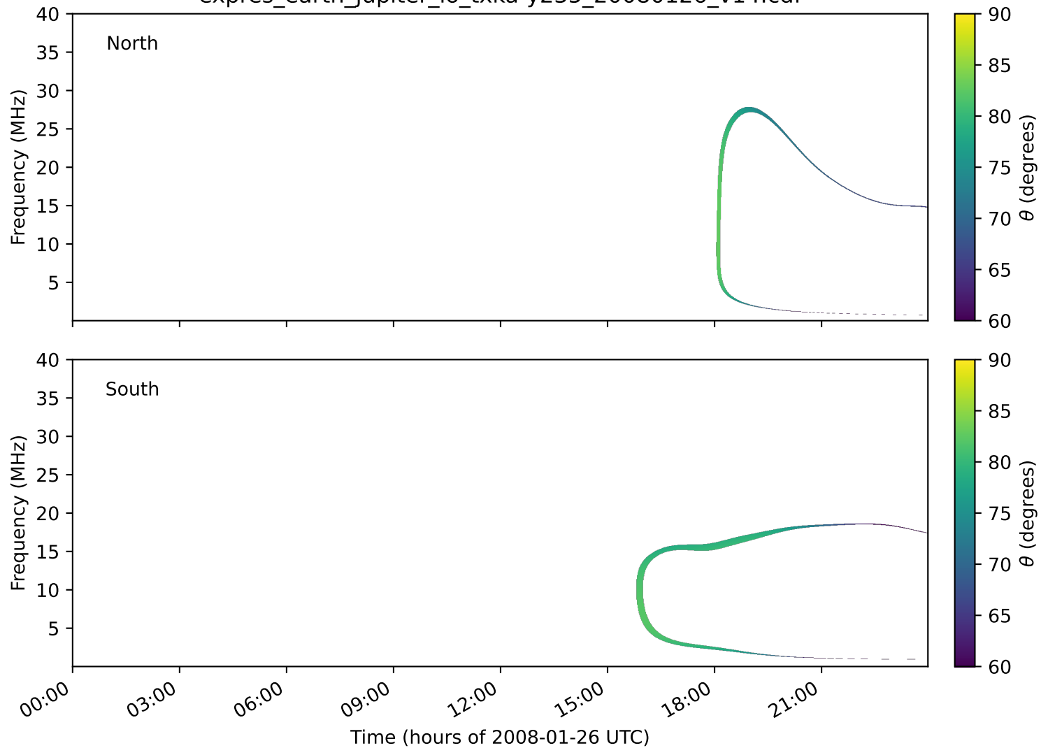
expres_earth_jupiter_io_txka-y235_20080126_v14.cdf
