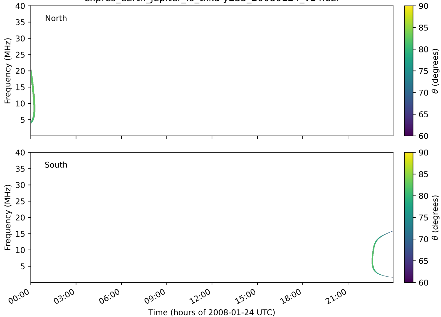
expres_earth_jupiter_io_txka-y235_20080124_v14.cdf
