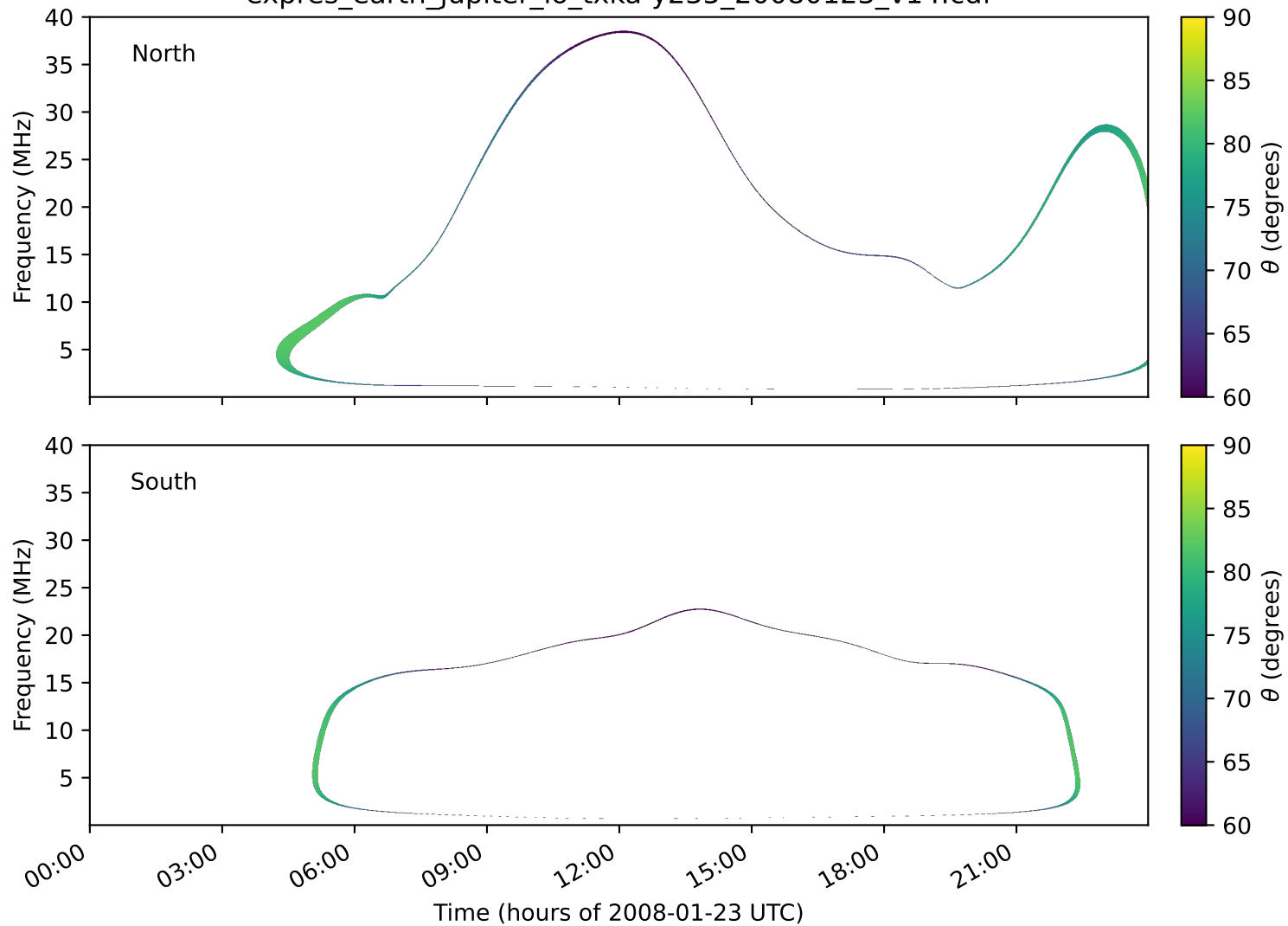
expres_earth_jupiter_io_txka-y235_20080123_v14.cdf
