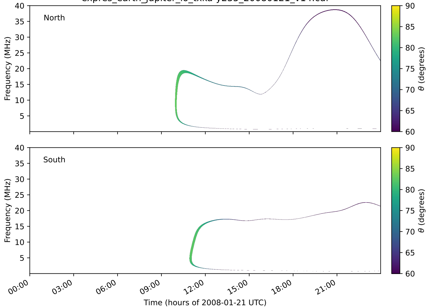
expres_earth_jupiter_io_txka-y235_20080121_v14.cdf
