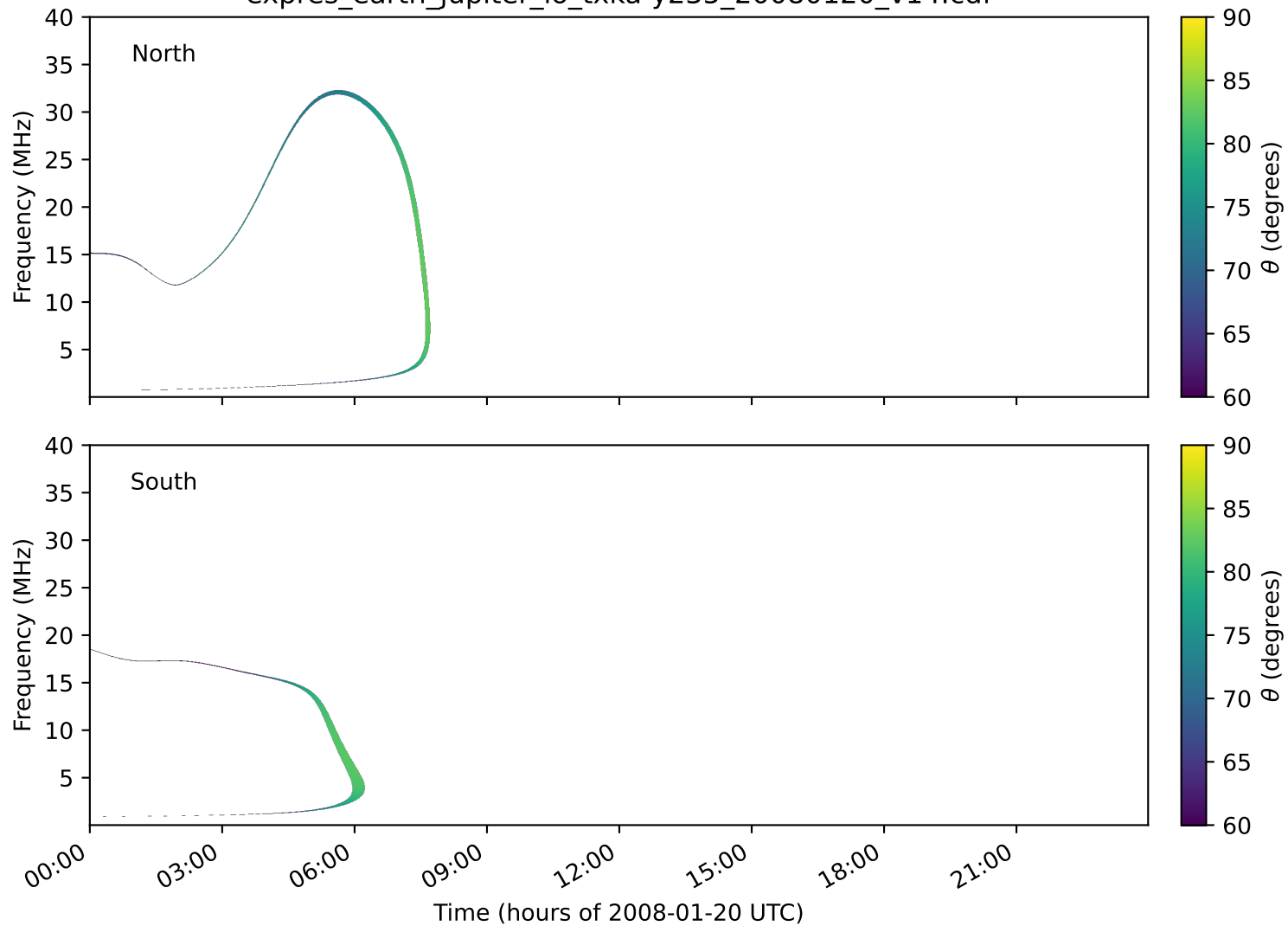
expres_earth_jupiter_io_txka-y235_20080120_v14.cdf
