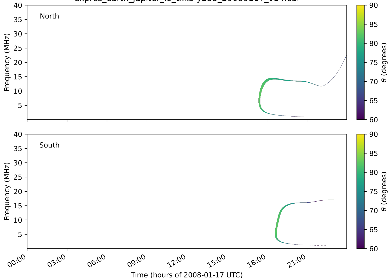
expres_earth_jupiter_io_txka-y235_20080117_v14.cdf
