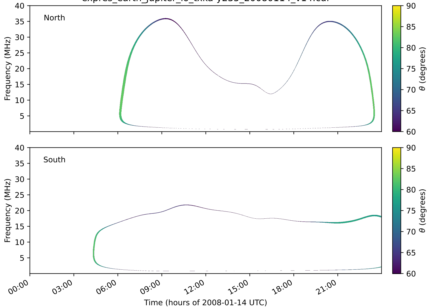
expres_earth_jupiter_io_txka-y235_20080114_v14.cdf
