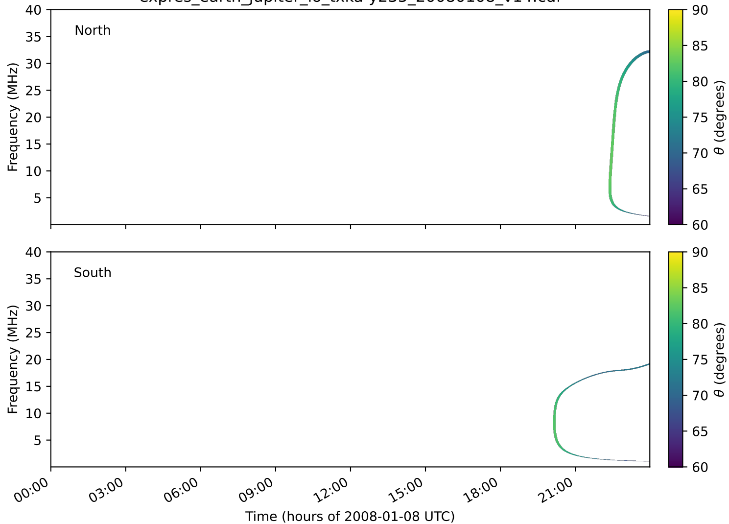
expres_earth_jupiter_io_txka-y235_20080108_v14.cdf
