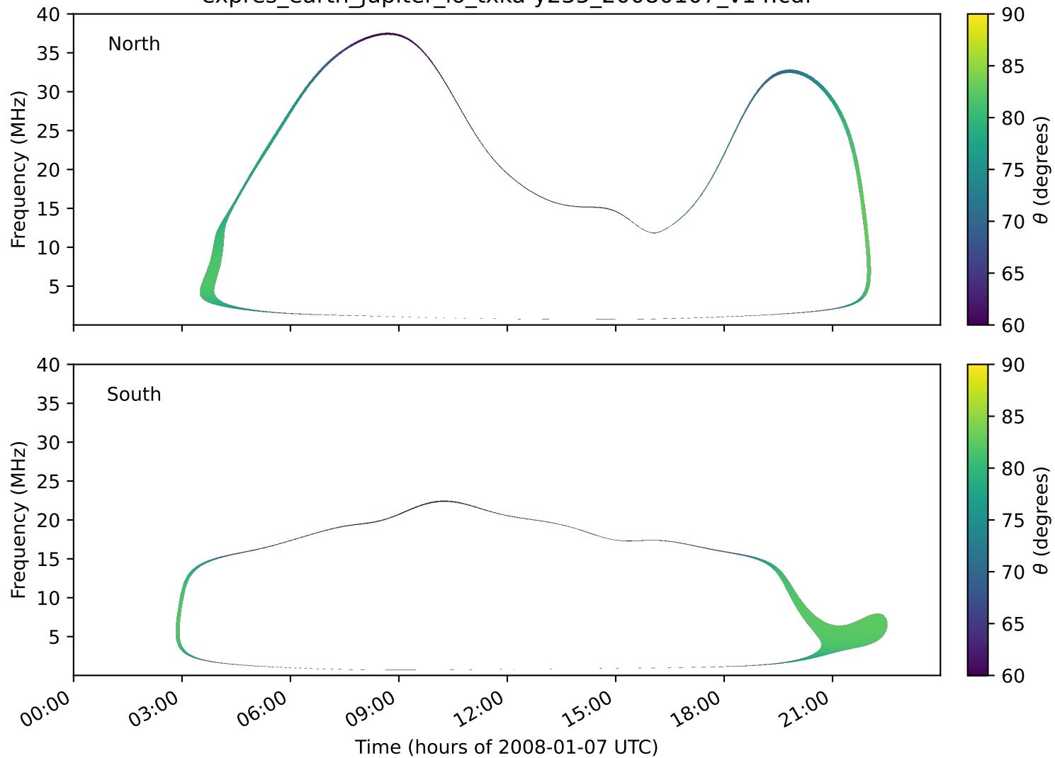
expres_earth_jupiter_io_txka-y235_20080107_v14.cdf
