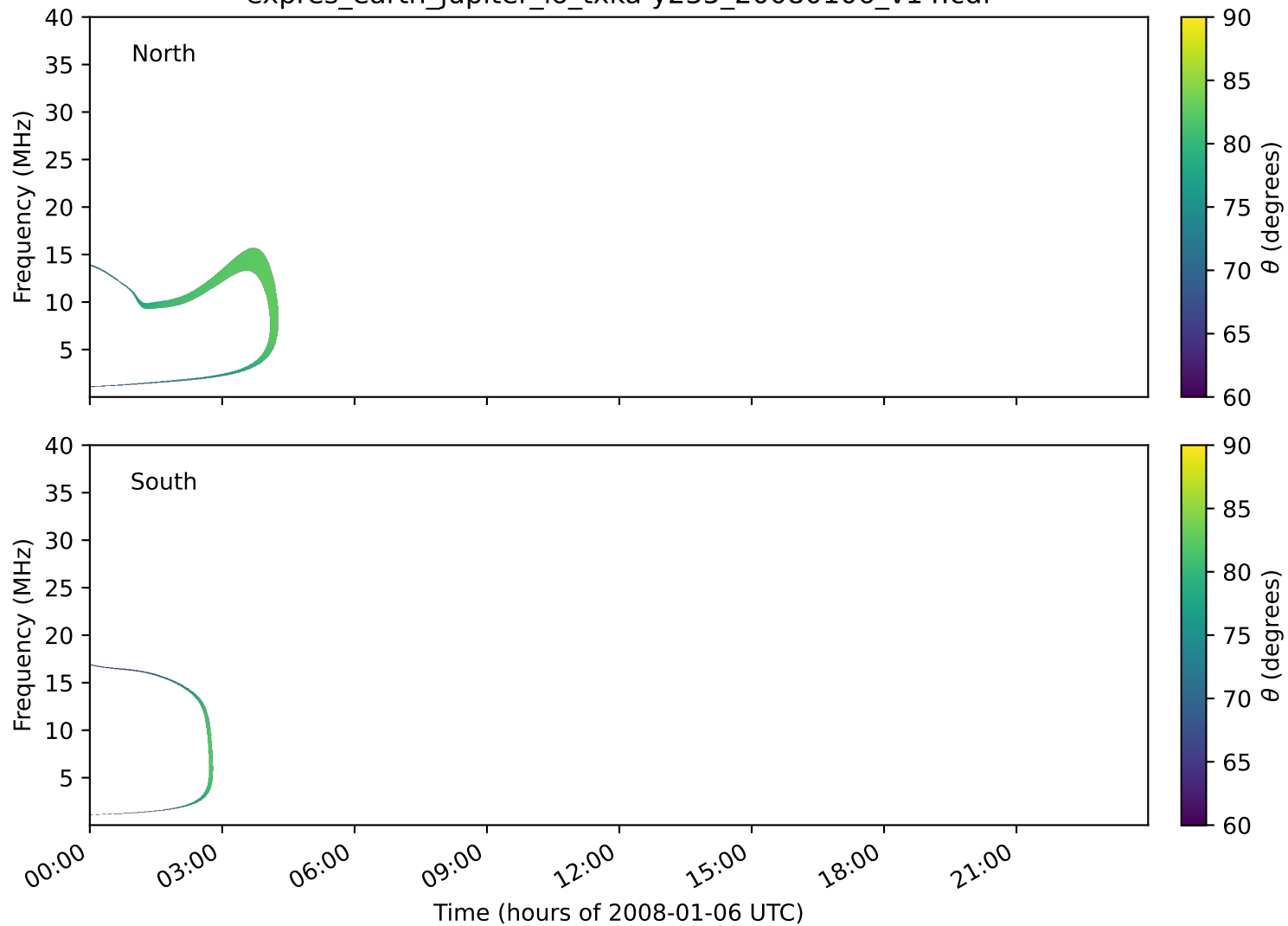
expres_earth_jupiter_io_txka-y235_20080106_v14.cdf
